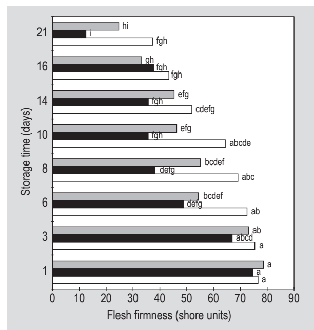
Figure 2. Effect of different kafirin based coatings on flesh texture (as determined by densitometer) of avocados stored at 18 °C for 21 days. Black bars = no coating; grey bars = kafirin propylene glycol (PG) coating; white bars = kafirin-PG + glucono-delta-lactone coating. Mean values with different lower case letters differ significantly from each other (treatment × day: P=0.002 ).
