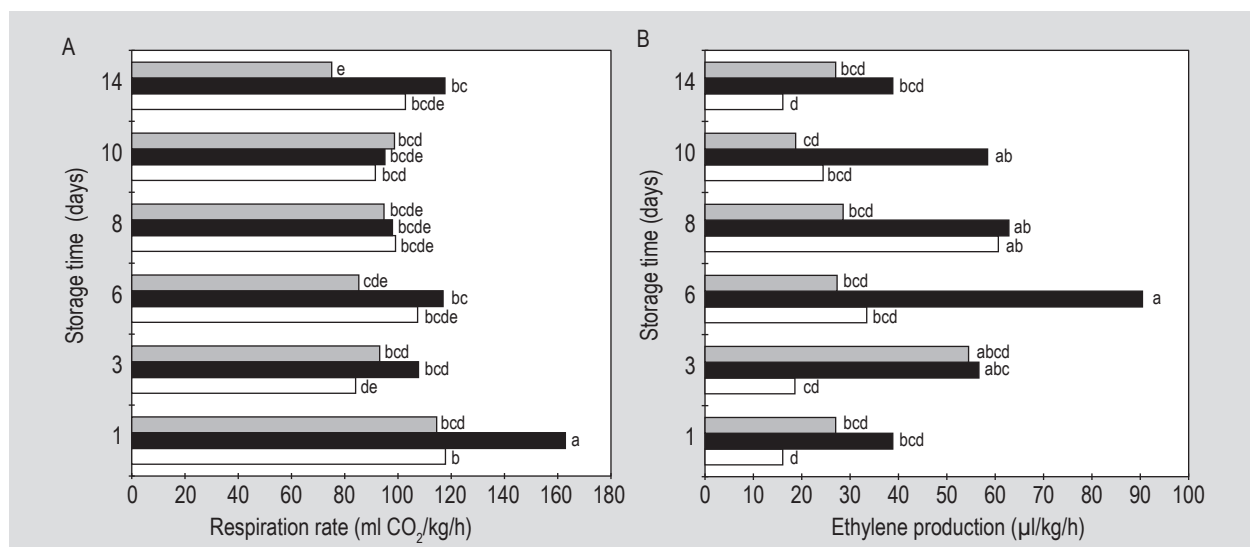
Figure 1. Effect of different kafirin based coatings on the respiration rate and ethylene production of avocados stored at 18 °C for 14 days. (A) Respiration rate. (B) Ethylene production. Black bars = no coating; grey bars = kafirin propylene glycol (PG) coating; white bars = kafirin-PG + glucono-delta-lactone coating. Mean values with different lower case letters differ significantly from each other (treatment \times day: P < 0.0001 ).
