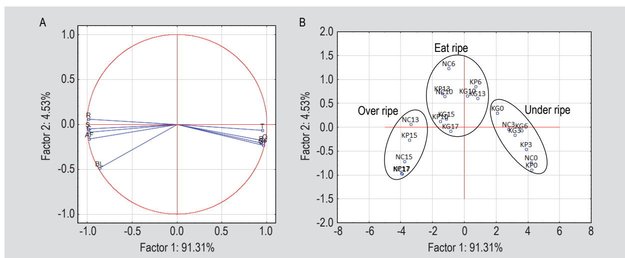
Figure 3. Principal component analysis loadings for (A) sensory attributes and flesh firmness measured by densitometer during ripening and (B) all coated and uncoated avocados analysed on day 0, 3, 6, 10, 13, 15, and day 17 of the shelf-life study. NC = no coating; KP = kafirin-propylene glycol (PG); KG = kafirin-PG + glucono-delta-lactone; R = visual extent of ripeness; S = softness; C = creaminess; AF = avocado flavour (flavour intensity); BL = presence of dark flesh blemishes; T = flesh firmness; O = oiliness (fatty); B = bitter aftertaste; GF = green flavour.
